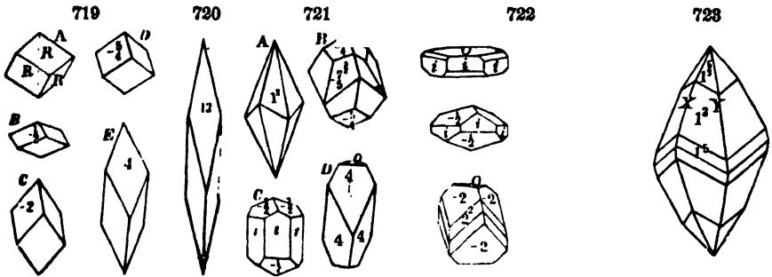
ANGLES OF RHOMBOHEDRONS
